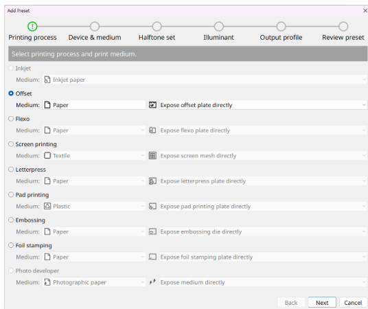
User interface for adding a preset
