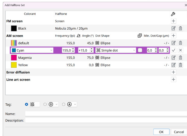
User interface for adding a halftone set
