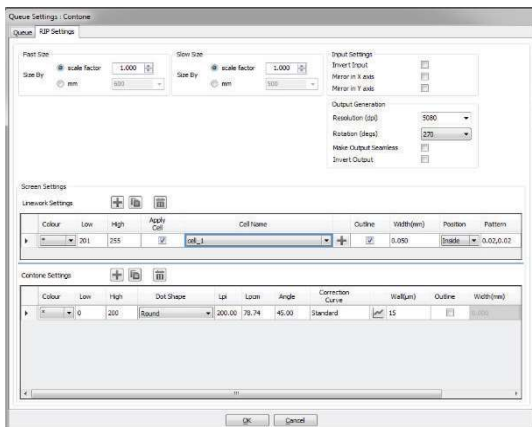
User interface for raster settings
